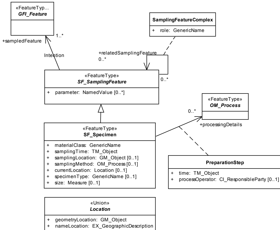
Figure 13— Specimen model
