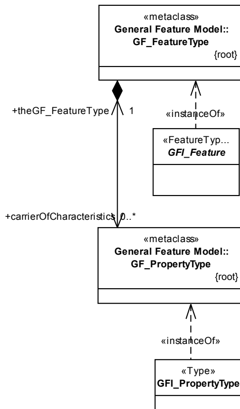
Figure 14—Feature Instance model
